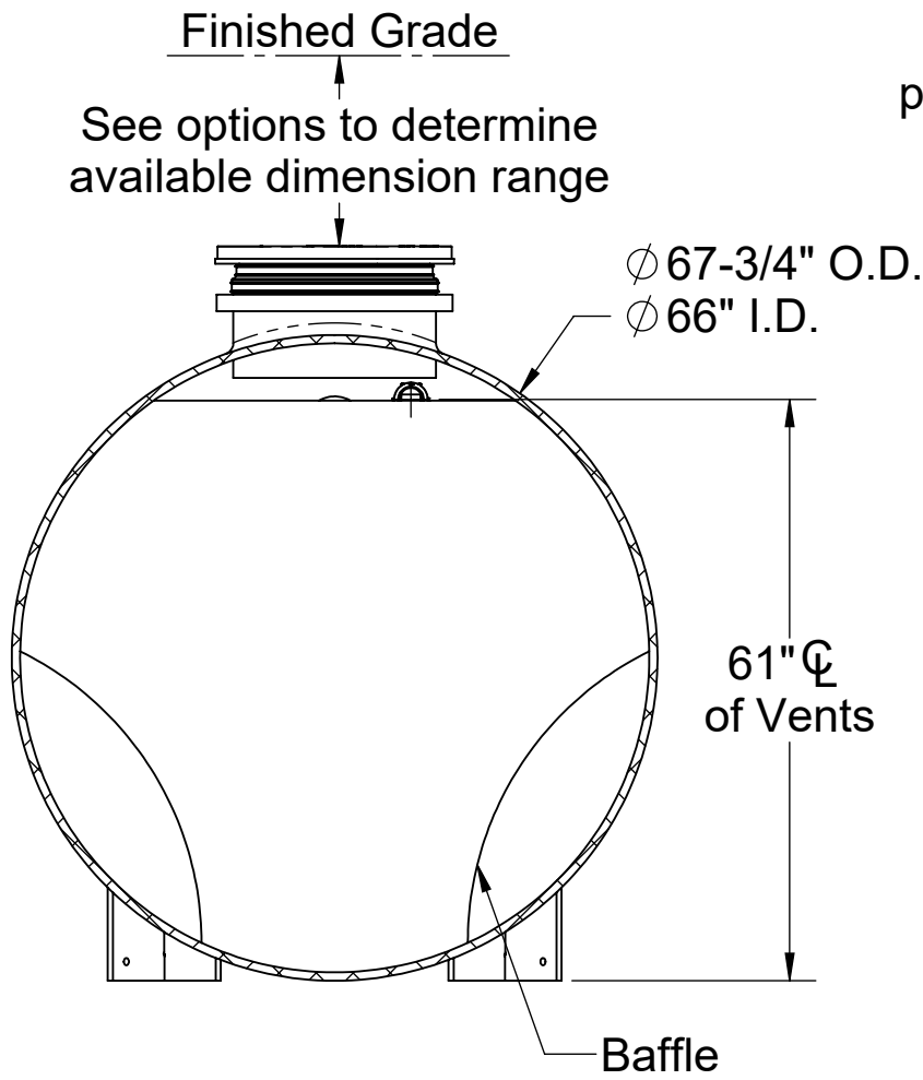
SECTION B-B
