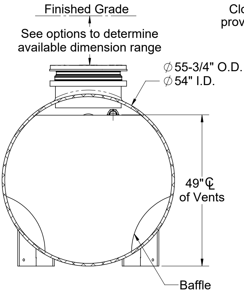
SECTION B-B
