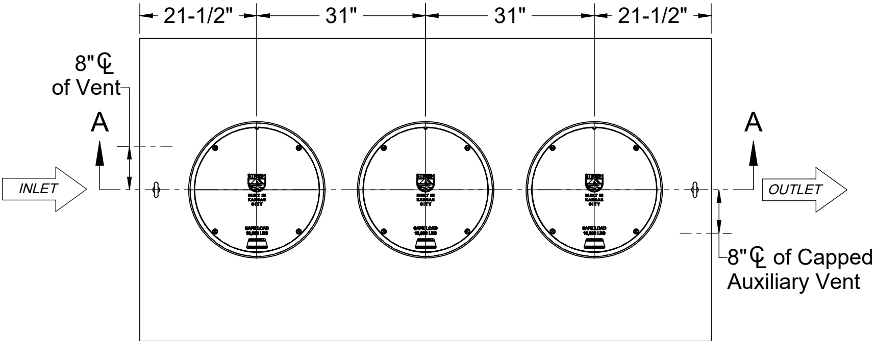
TOP VIEW
