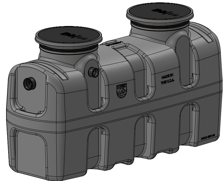
OS-350 OS SERIES 100 GPM High Efficiency Oil/Water Separator
