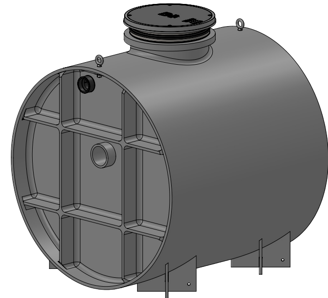
OS-500-OMAHA OS SERIES 475 GALLON OIL SEPARATOR
