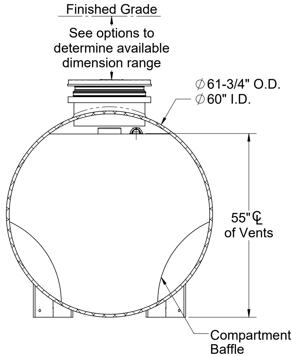
SECTION B-B
