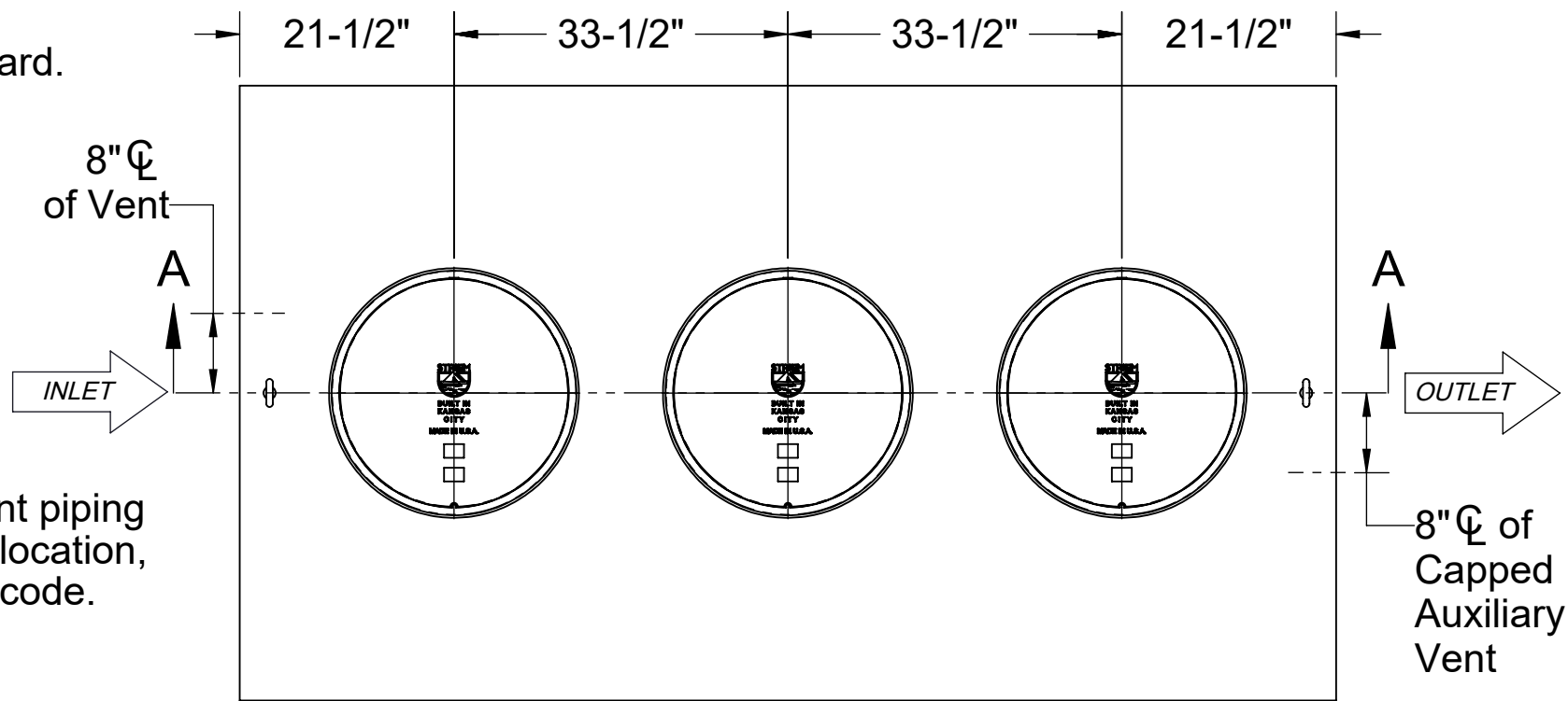
TOP VIEW
