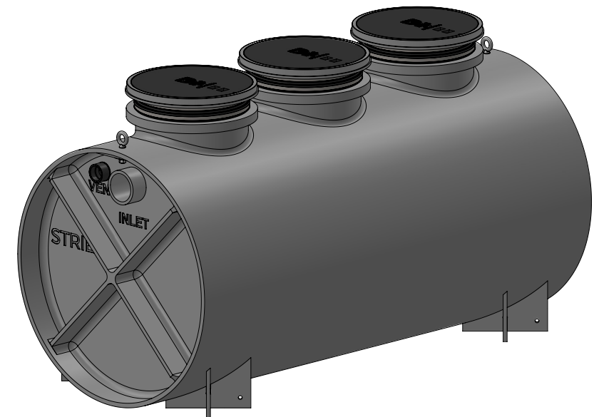
OT-500 OIL TANKER™ SERIES 562 GALLON OIL SEPARATOR
