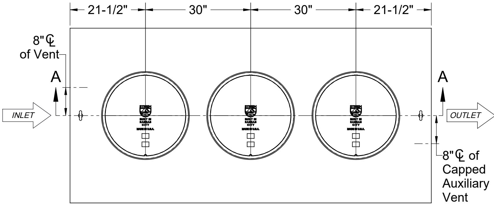
TOP VIEW
