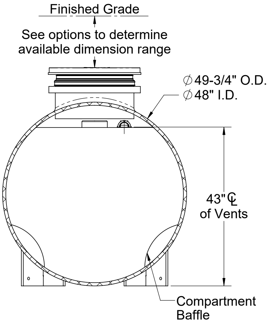
SECTION B-B
