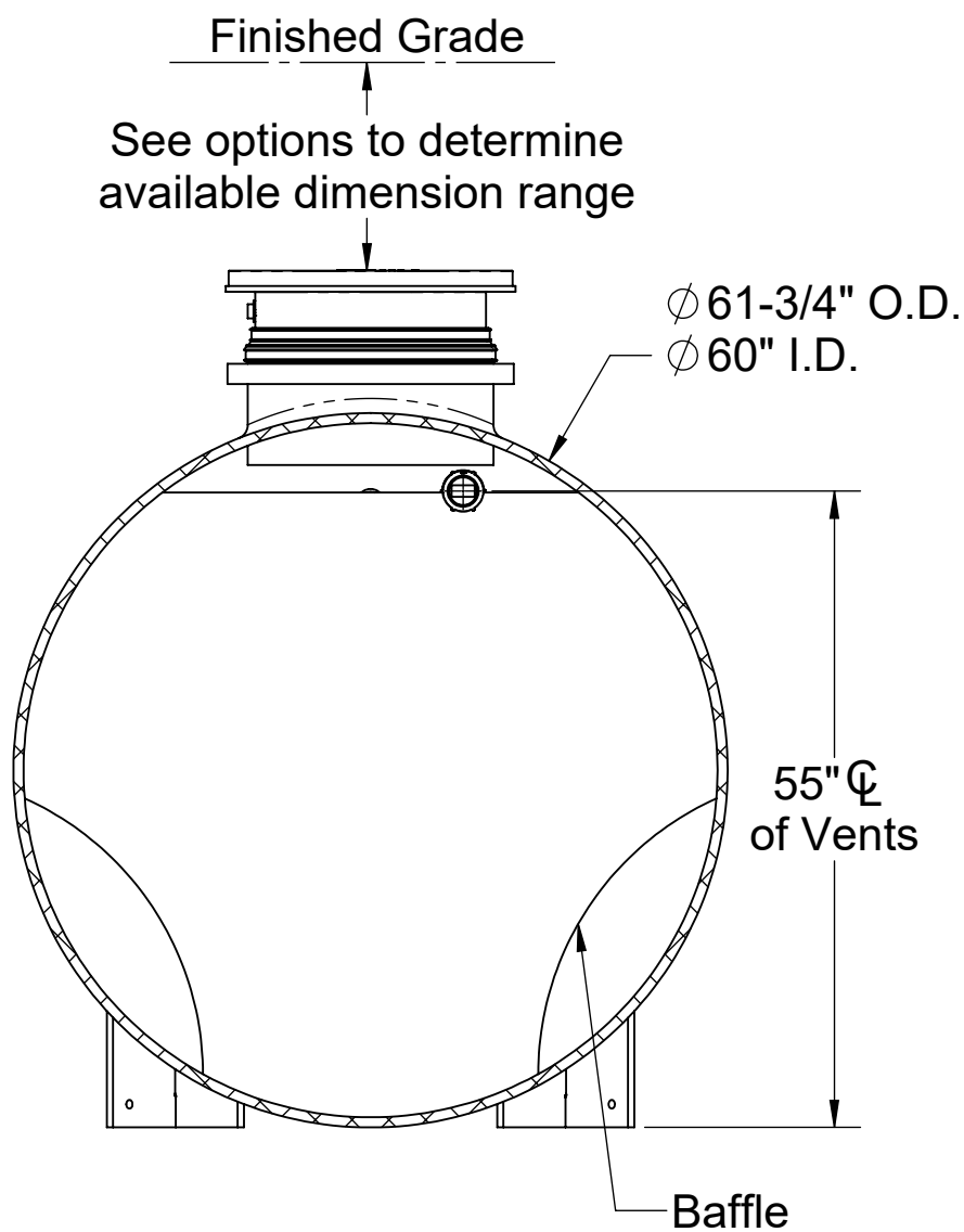
SECTION B-B
