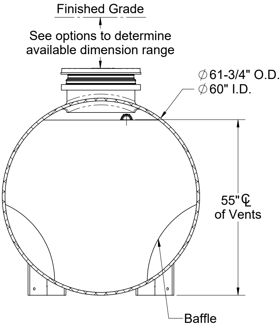
SECTION B-B
