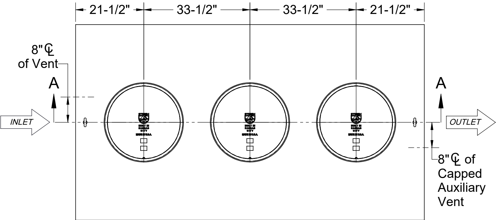
TOP VIEW
