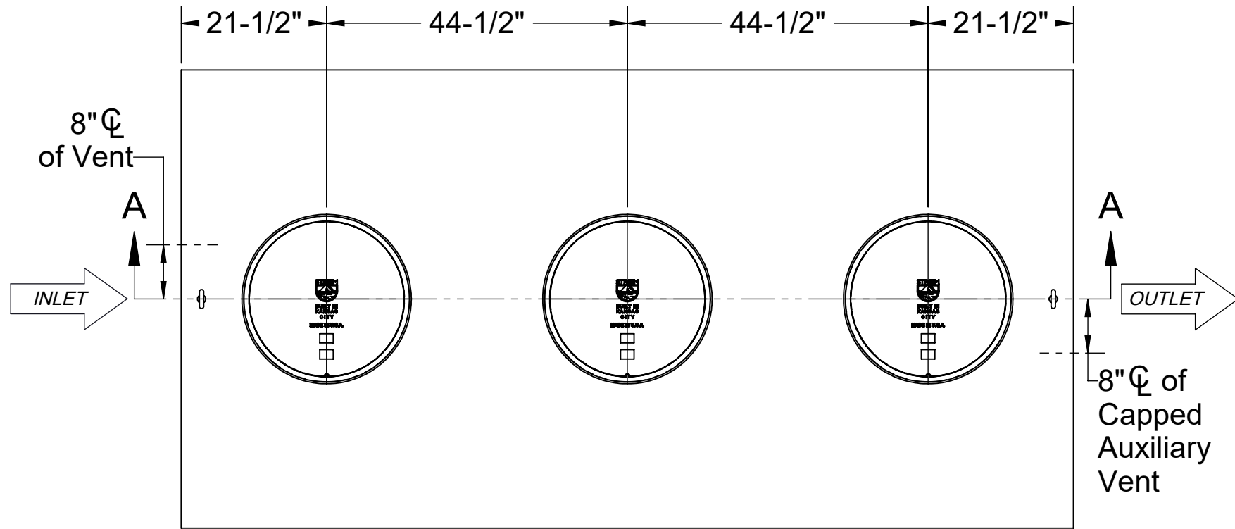
TOP VIEW
