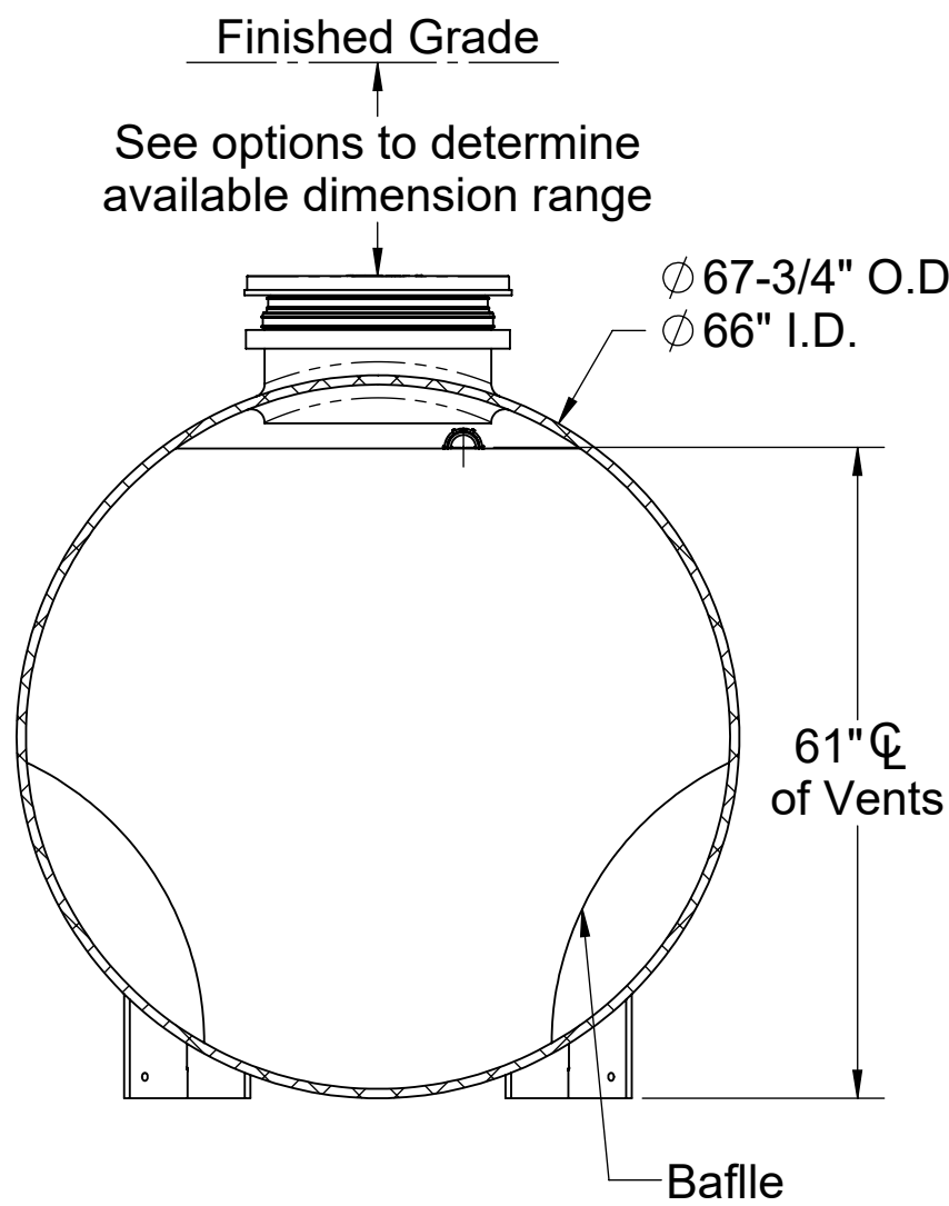
SECTION B-B
