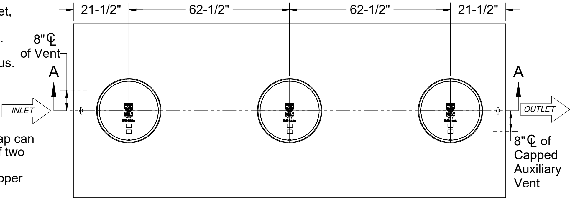
TOP VIEW
