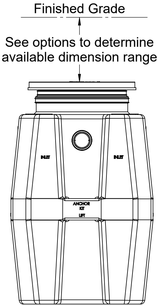
END VIEW
