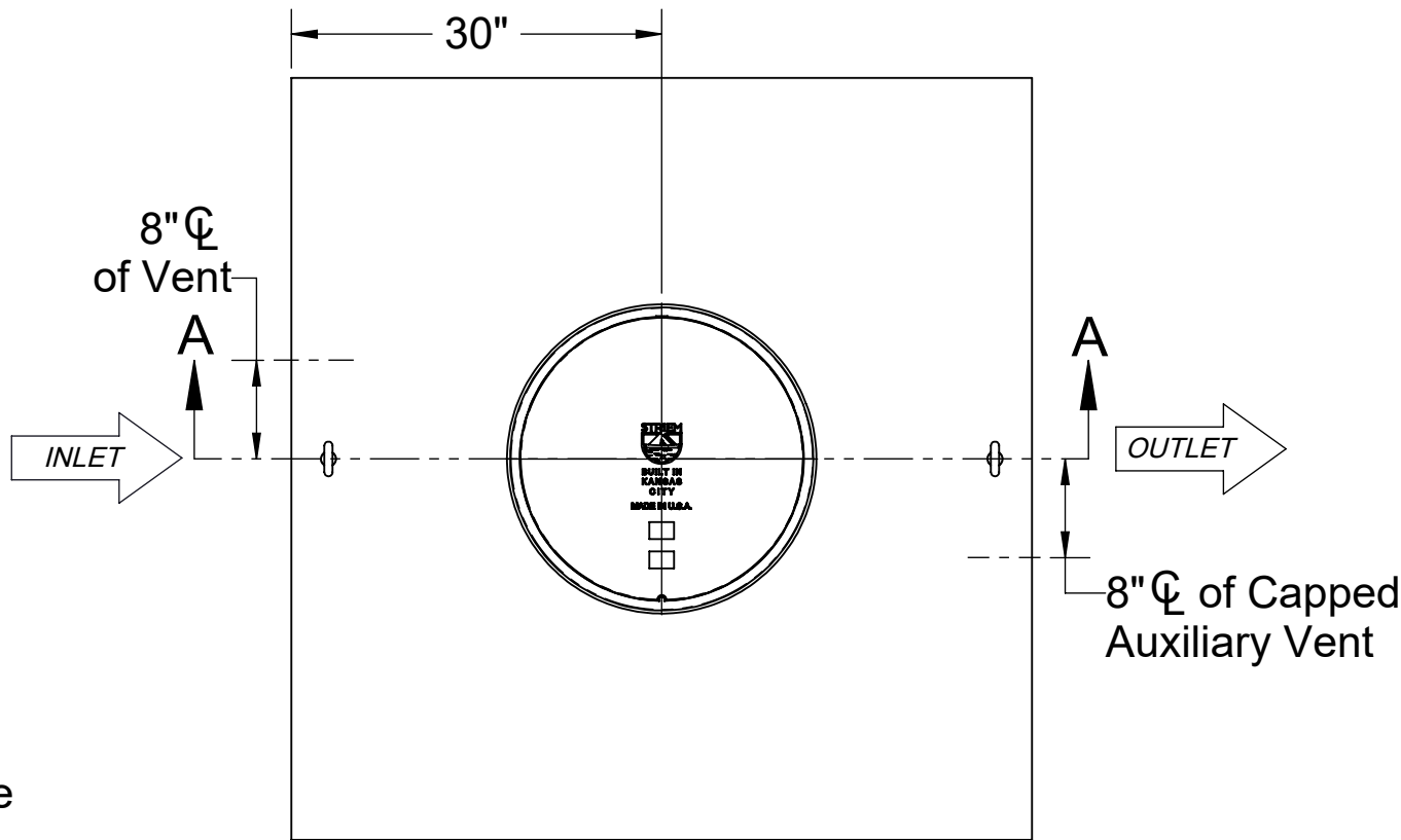
TOP VIEW
