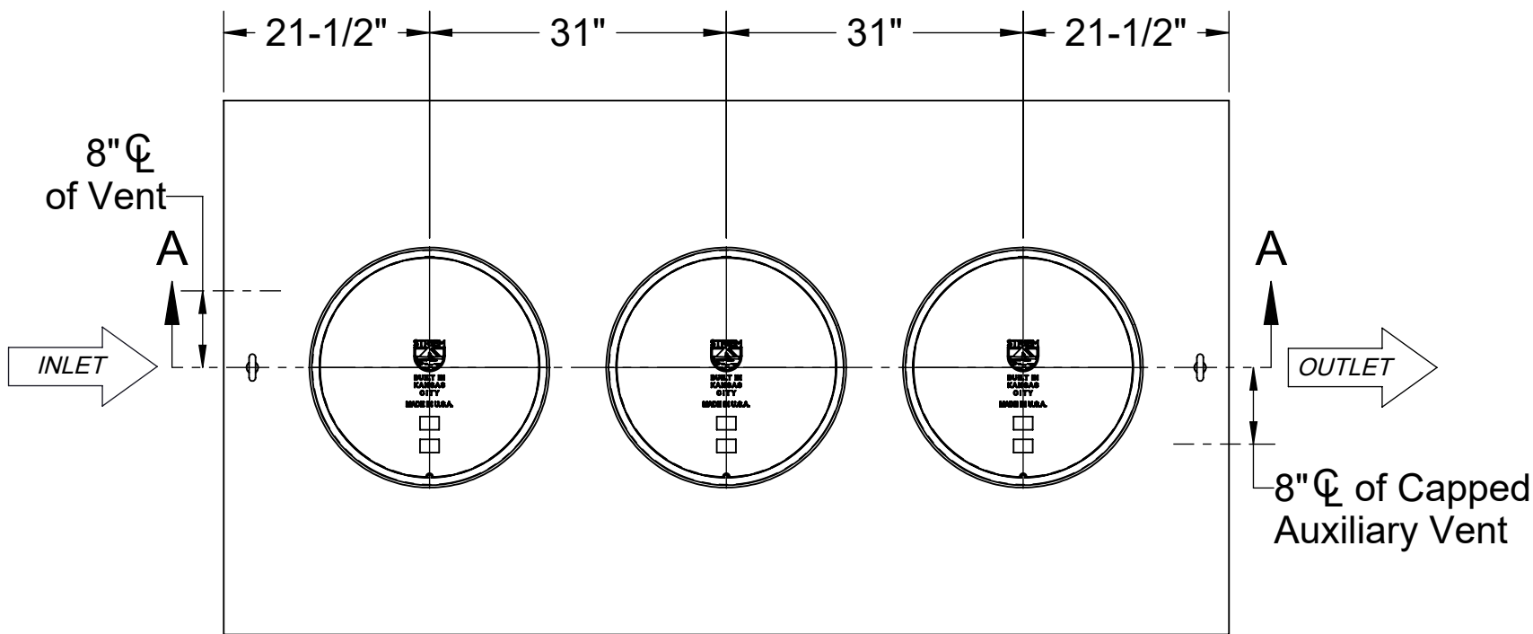
TOP VIEW
