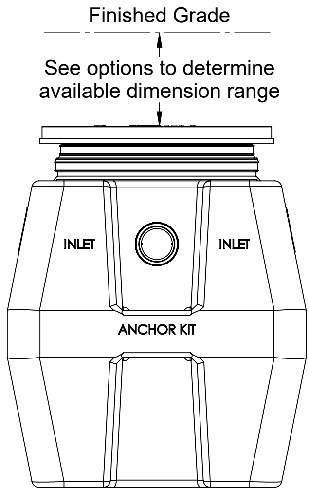
END VIEW
