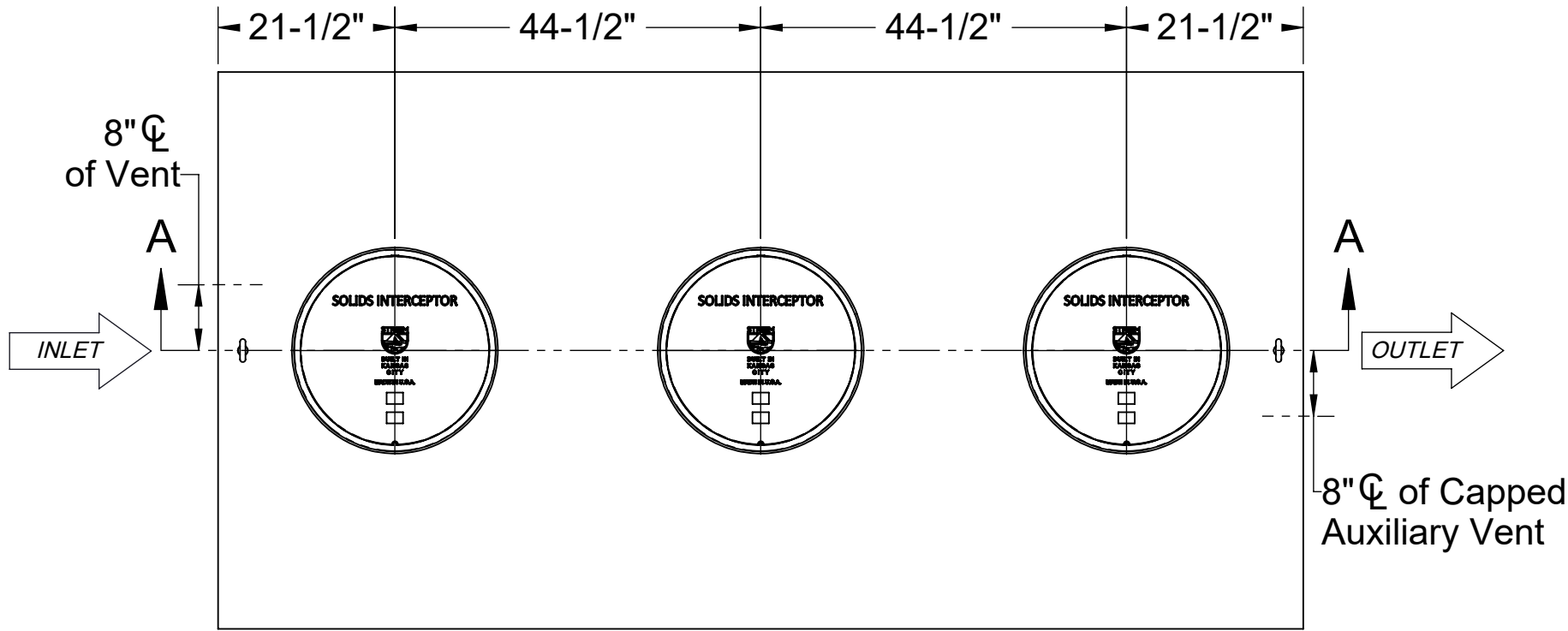
TOP VIEW
