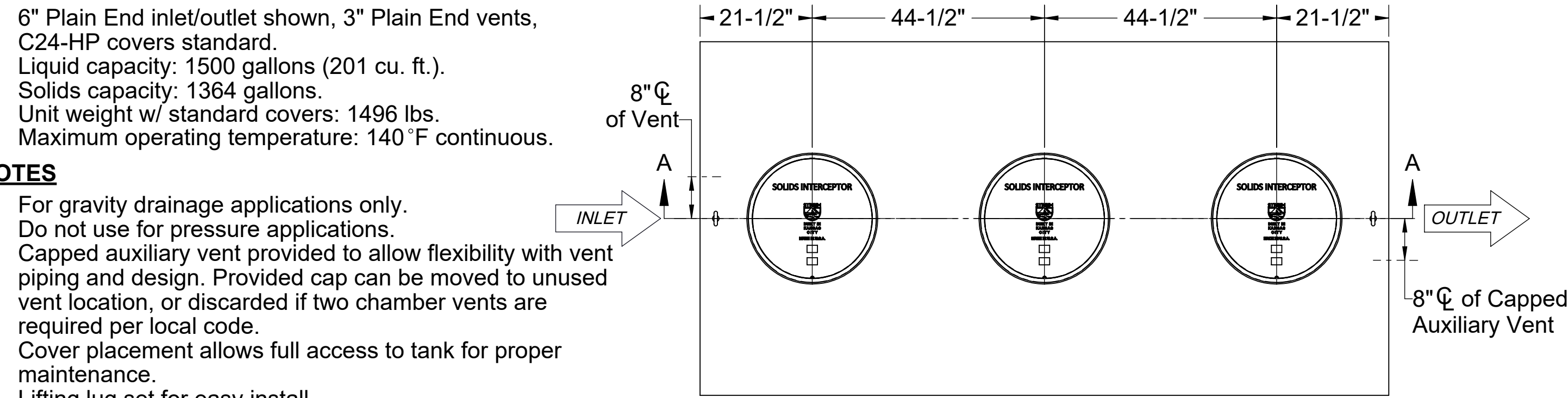
TOP VIEW
