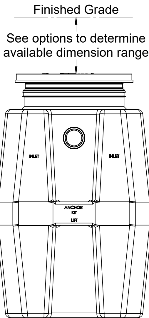
END VIEW
