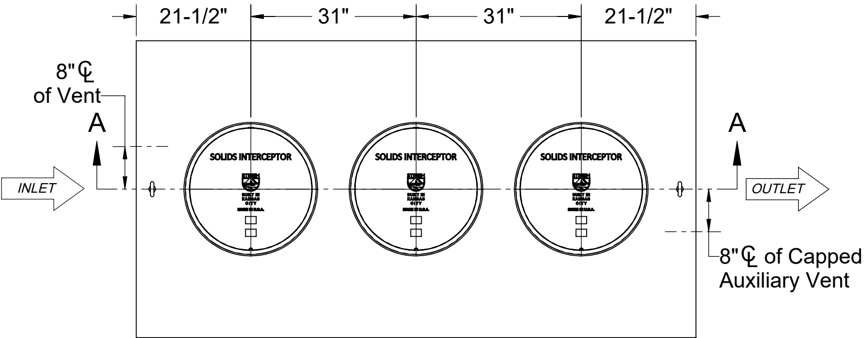
TOP VIEW
