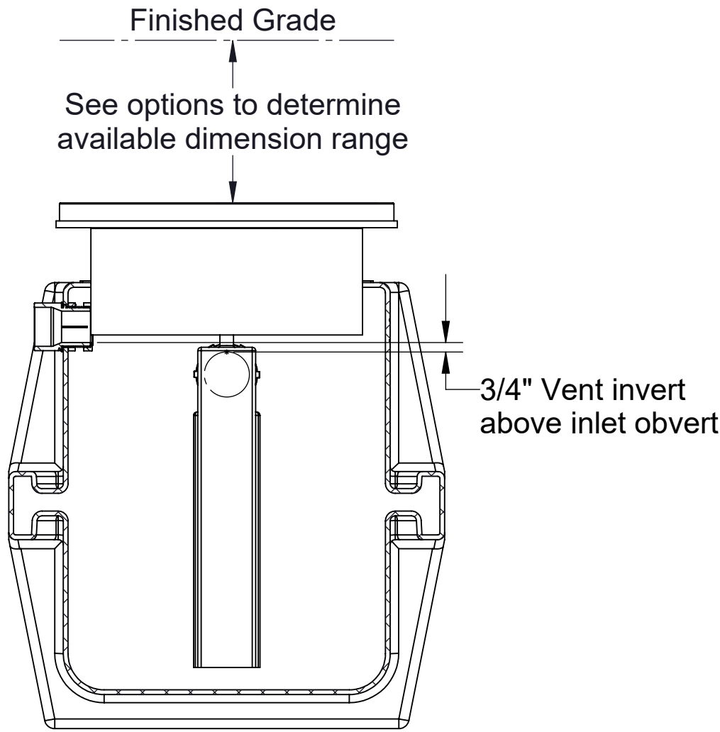
SECTION B-B
