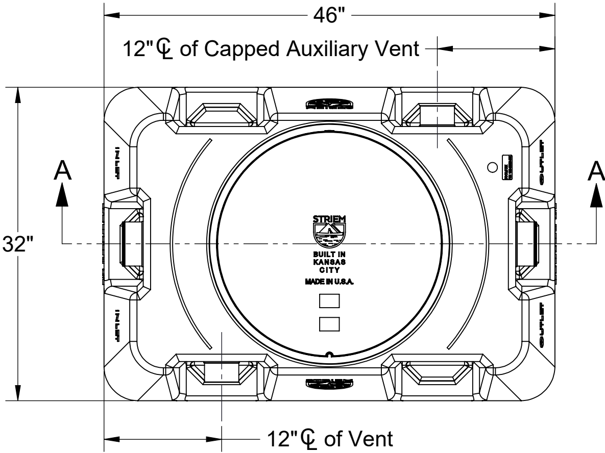
TOP VIEW
