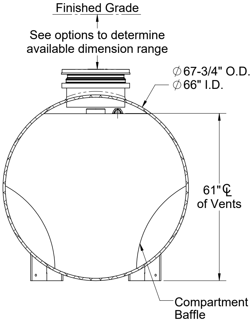
SECTION B-B
