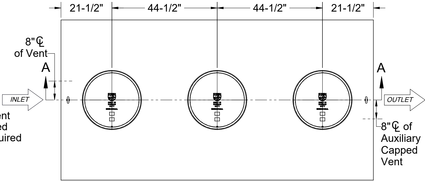
TOP VIEW
