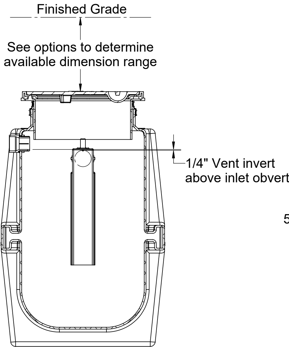
SECTION B-B
