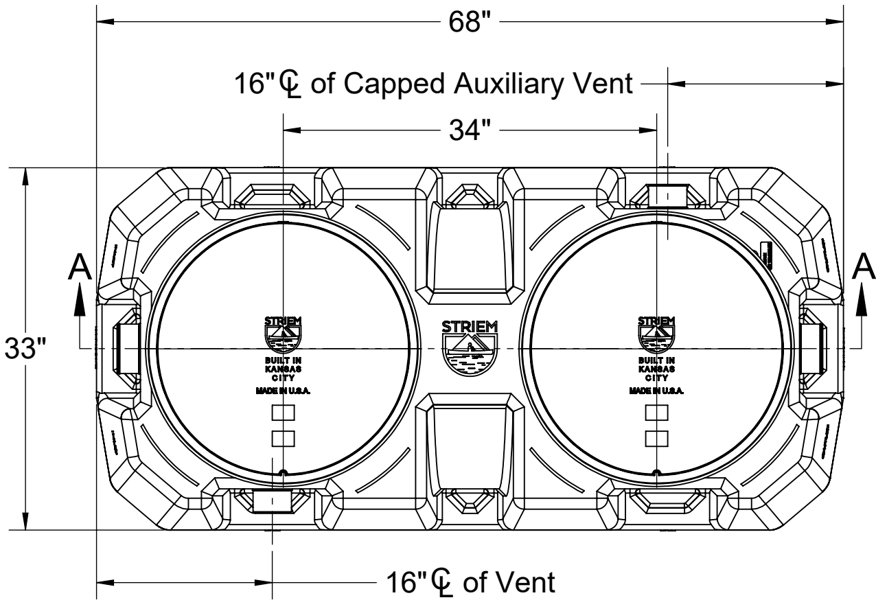
TOP VIEW
