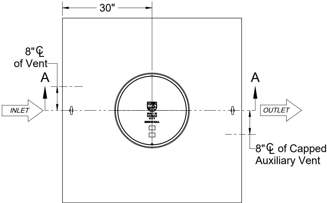
TOP VIEW
