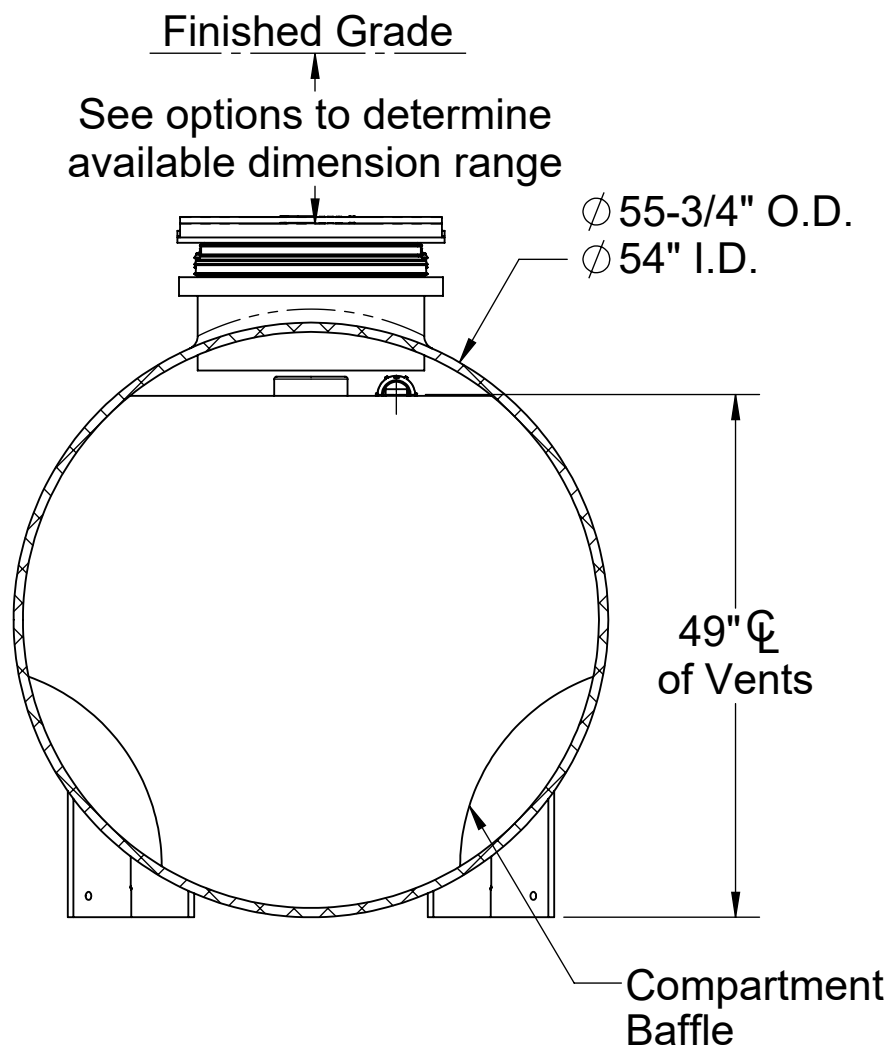
SECTION B-B
