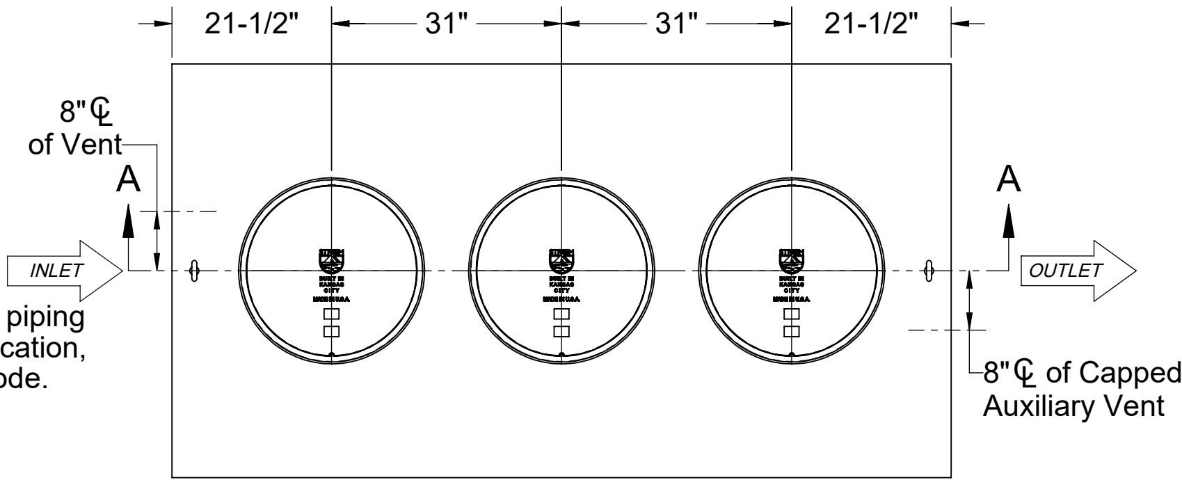
TOP VIEW
