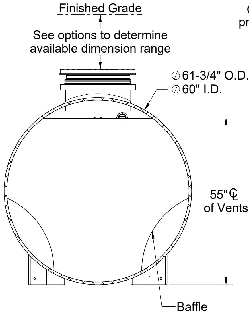
SECTION B-B
