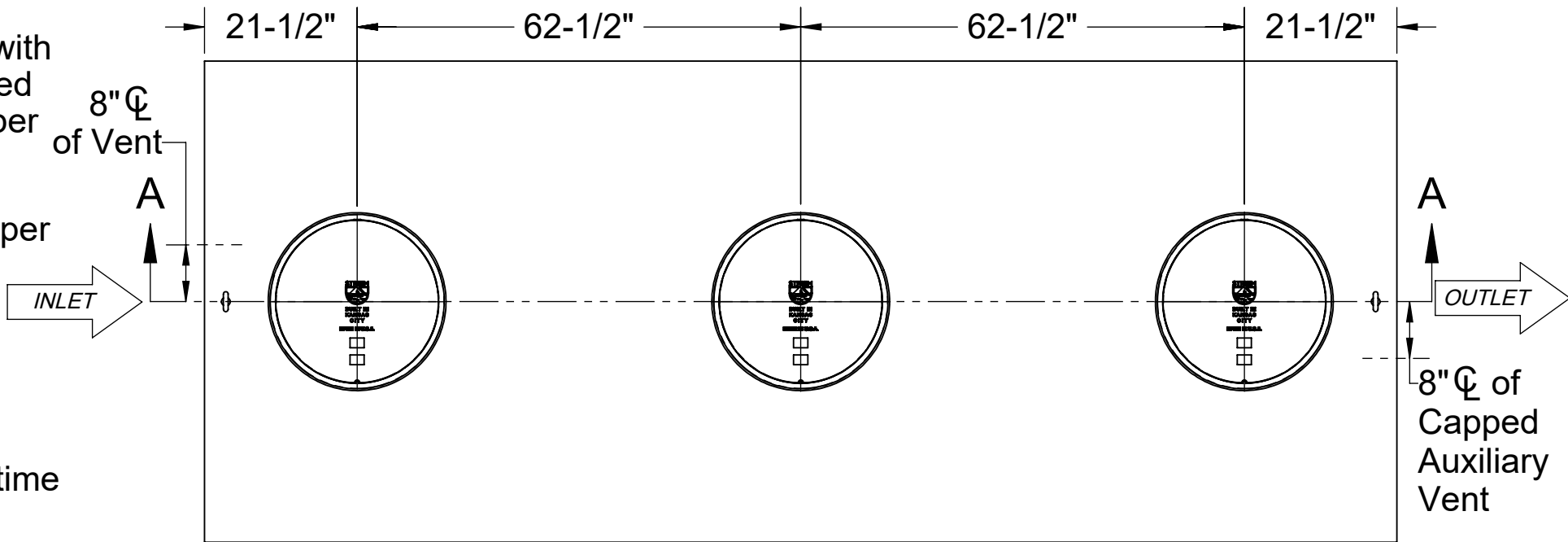
TOP VIEW
