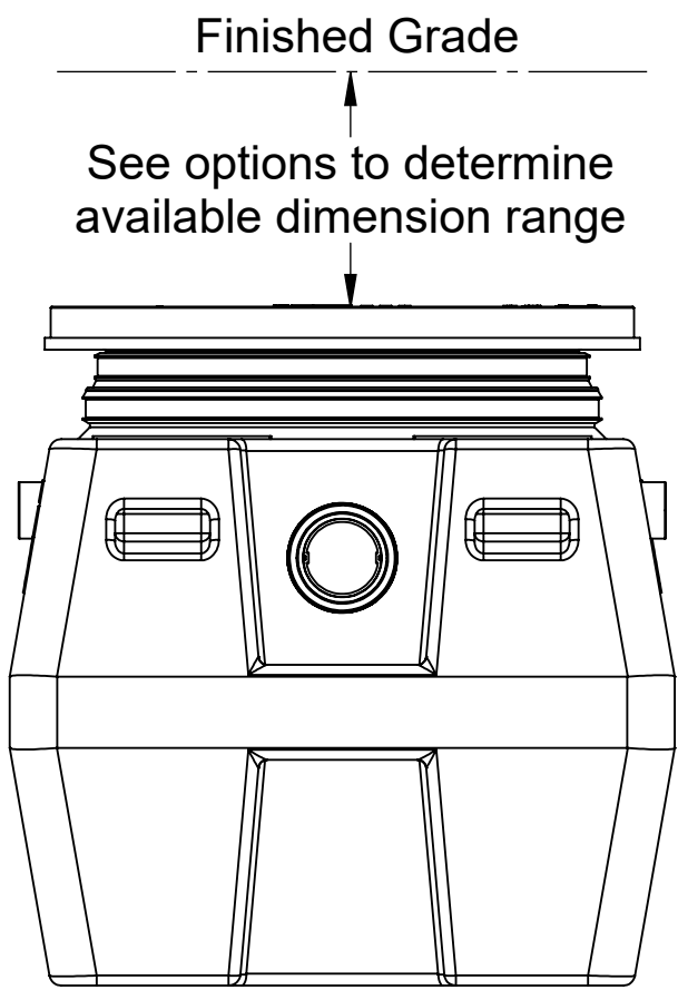
END VIEW
