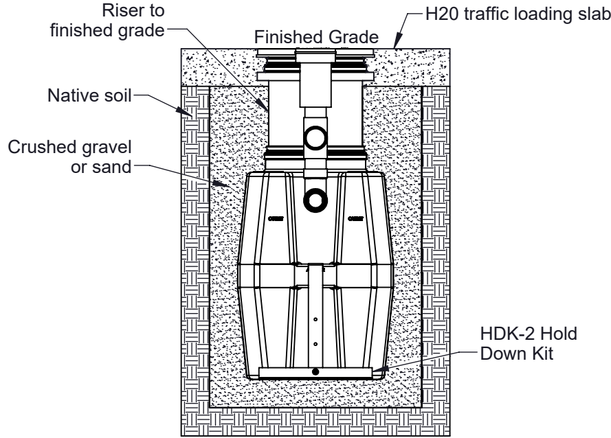
EXCAVATION AND BACKFILL DETAIL
