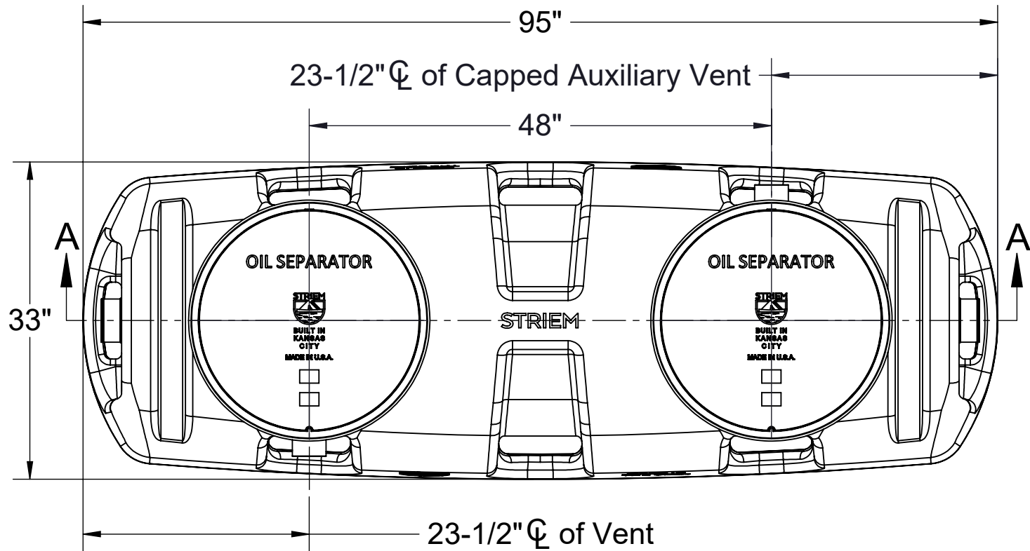
TOP VIEW
