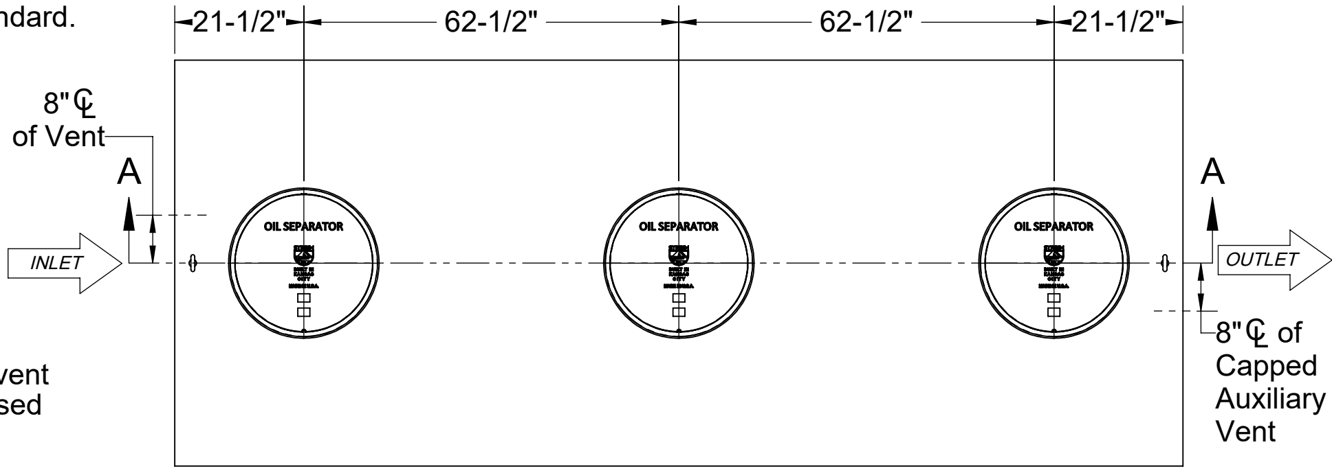
TOP VIEW
