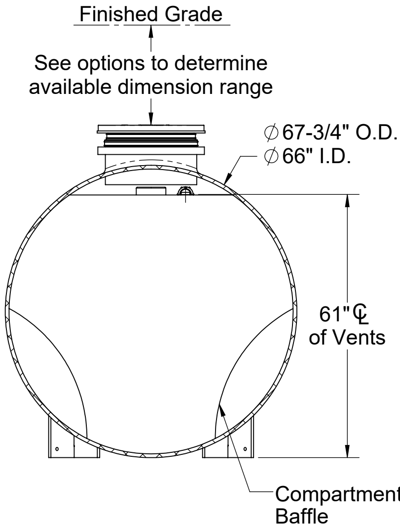
SECTION B-B
