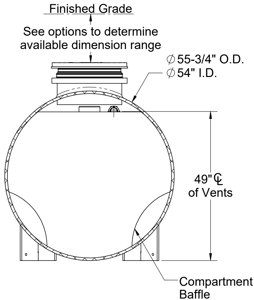
SECTION B-B
