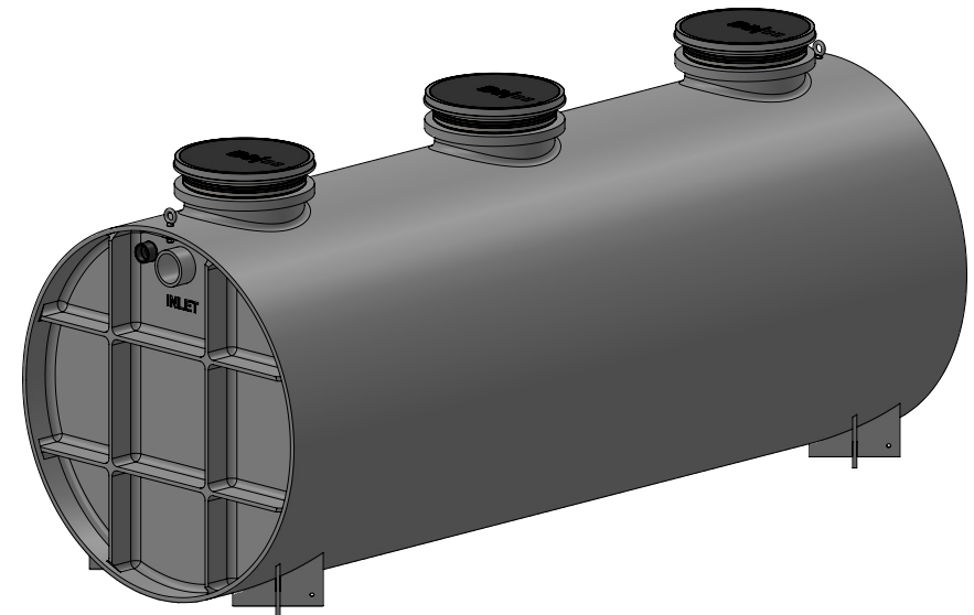
FLI-2000 FLAMMABLE LIQUID INTERCEPTOR 2,000 GAL
