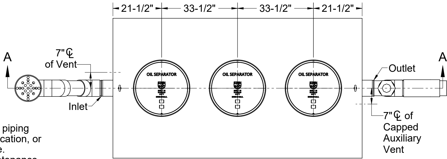
TOP VIEW
