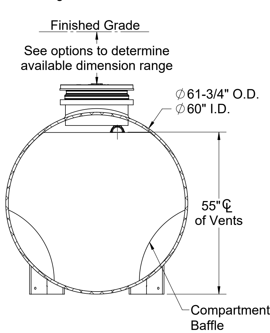
SECTION B-B
