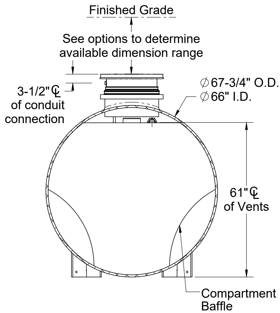
SECTION B-B
