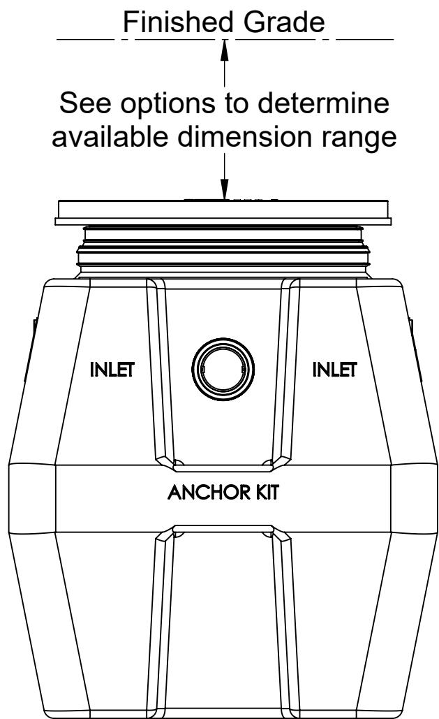
END VIEW
