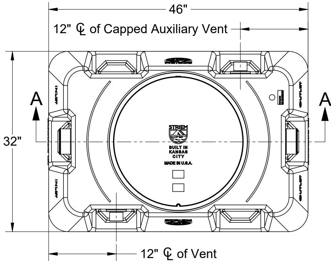
TOP VIEW
