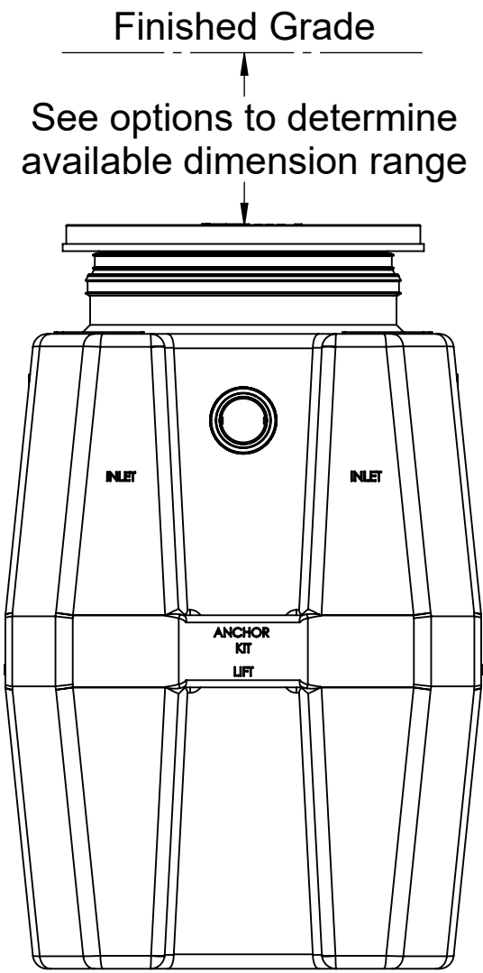
END VIEW
